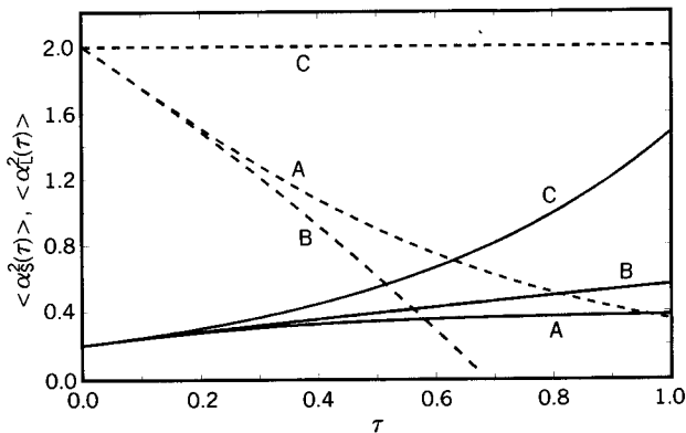
Figure 8. Time dependence of \langle \hat{\alpha}_S^2(\tau) \rangle = \langle \alpha_S^2(\tau) \rangle (solid lines) and \langle \hat{\alpha}_L^2(\tau) \rangle = \langle \alpha_L^2(\tau) \rangle (dashed lines) for the same cases as in Fig. 7.
